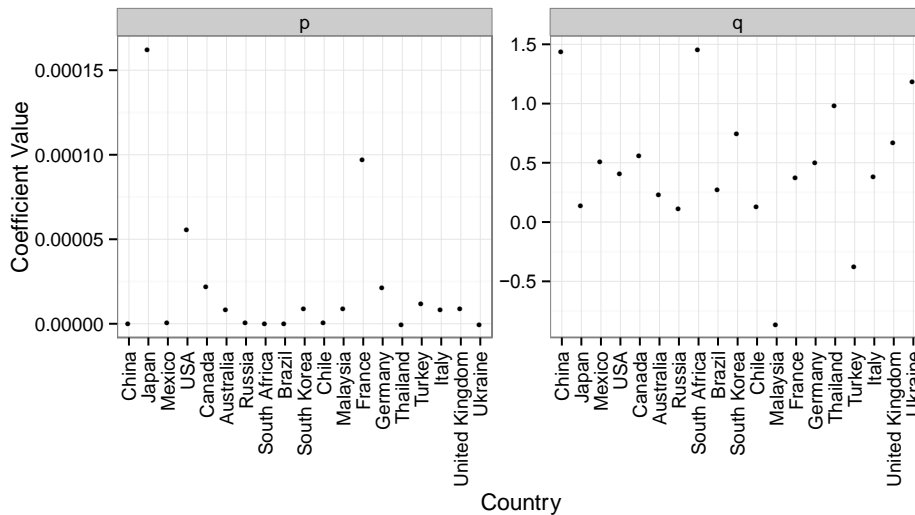
Figure 20: Coefficients from Bass model calibrated to historical sales of full battery electric vehicles. The p coefficient describes the coefficient of innovation, the higher this value the greater the initial uptake of the technology when initially offered. The q coefficient describes the coefficient of imitation, the higher this value the greater the growth of the technology after the “first-takers” have been saturated.
