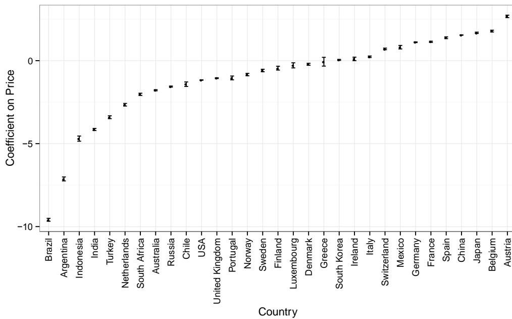
Figure 16: Relative price ($100,000s) odds-ratio coefficients from discrete choice logit models run independently for 31 countries. Price sensitivity decreases from left to right.
