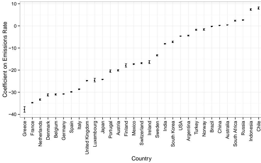
Figure 18: Relative emissions rate (mg CO 2 /km) in odds-ratio coefficients from discrete choice logit models run independently for 31 countries.
