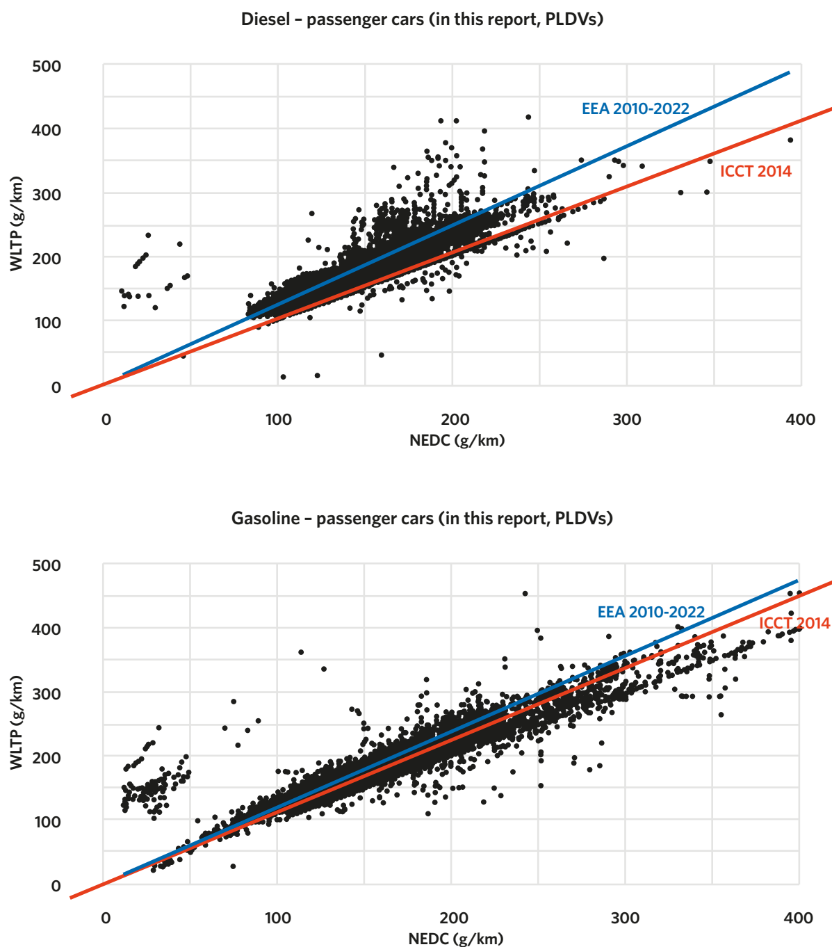
FIGURE A4: Powertrain-specific zero-intercept regressions between NEDC and WLTC, based on EEA data from 2019-2022
